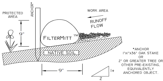
FILTERMITT™ OVERLAP END VIEW
