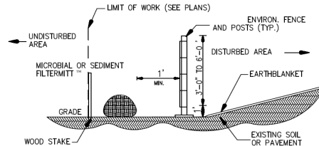
FENCE END ELEVATION 2:1 OR GREATER
