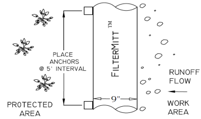
FILTERMITT™ OVERLAP TOP VIEW
